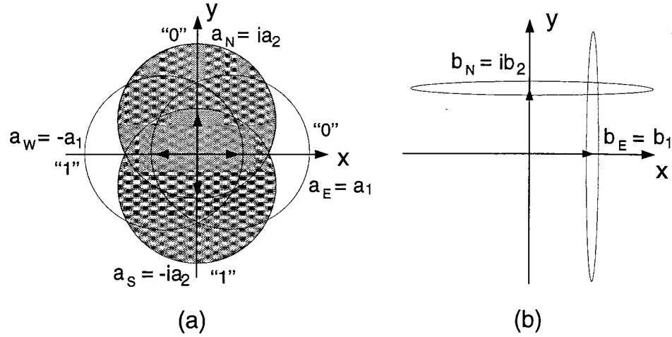
Fig. 2. On planes of quadrature-phase amplitudes, (a) shows Alice's encoding strategy based on four nonorthogonal coherent states; (b) shows Bob's tap-fibre modes using squeezed light. Uncertainty of a state is represented by error ellipses for squeezed states and by error circles for coherent states.
