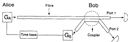
Fig. 1. The schematic diagram of the quantum cryptosystem using an optical coupler. Alice's (or sender's) signal generator is labeled by G_A ; Bob's (or receiver's) is labeled by G_B .
