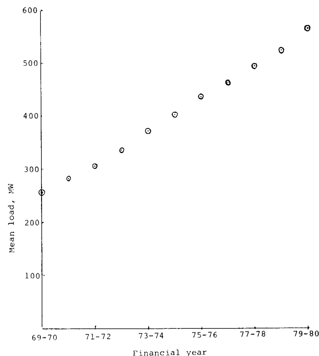
FIGURE 1 Mean electricity load in WA, in MW, for the 11 financial years 1969-70 to 1979-80. (The mean electricity load is the annual energy generated divided by 8760 hours.)
