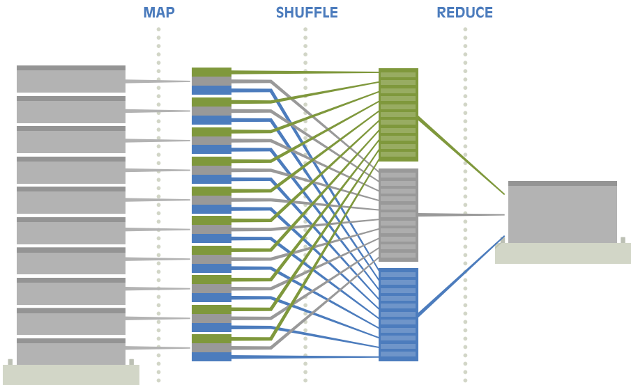
Figure 3: Map and Reduce Processing
