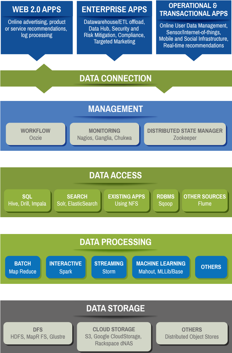
Figure 4: Hadoop's Ecosystem
