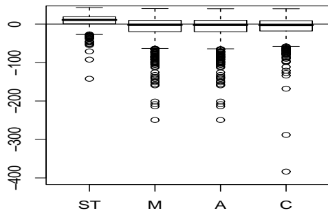
Scenario 1: Known lambda, Slope
