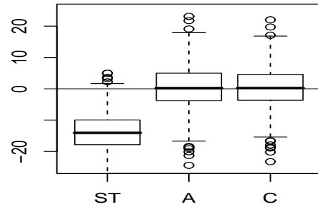
Scenario 2: Unknown lambda, Slope
