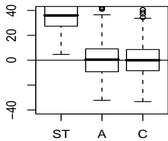
Scenario 2: Unknown lambda, Intercept
