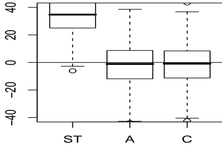
Scenario 2: Unknown lambda, Intercept
