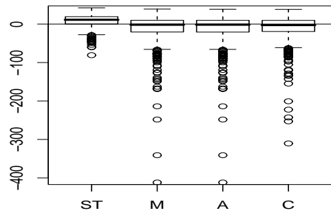
Scenario 1: Unknown lambda, Slope
