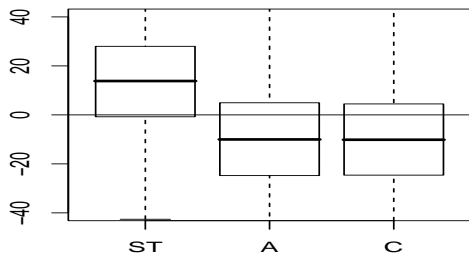
Scenario 2: Known lambda, Intercept
