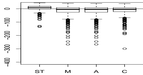
Scenario 2: Unknown lambda, Slope
