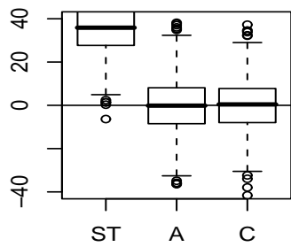
Scenario 2: Known lambda, Intercept
