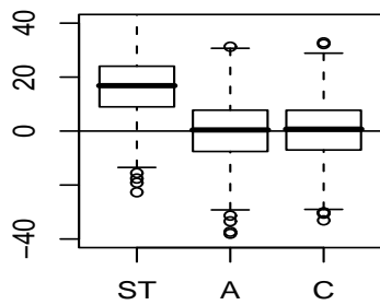
Scenario 1: Known lambda, Intercept
