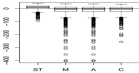
Scenario 2: Known lambda, Slope
