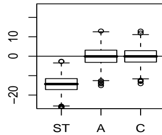
Scenario 2: Unknown lambda, Slope
