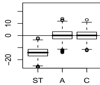
Scenario 2: Known lambda, Slope
