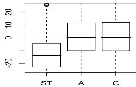
Scenario 2: Unknown lambda, Slope
