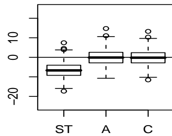
Scenario 1: Known lambda, Slope
