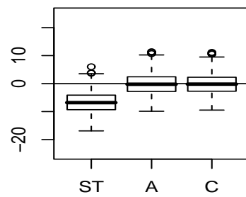
Scenario 1: Unknown lambda, Slope
