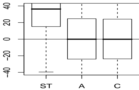
Scenario 2: Unknown lambda, Intercep
