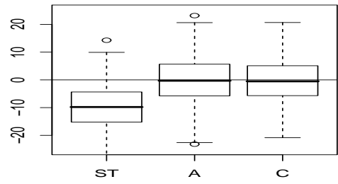
Scenario 2: Known lambda, Slope
