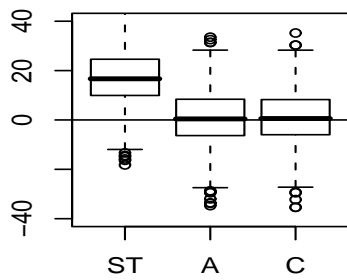
Scenario 1: Unknown lambda, Intercept
