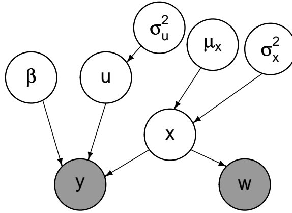
Figure 2: Directed acyclic graph representation of model (4), but with the predictor subject to measurement error. Shaded nodes correspond to the observed data.
