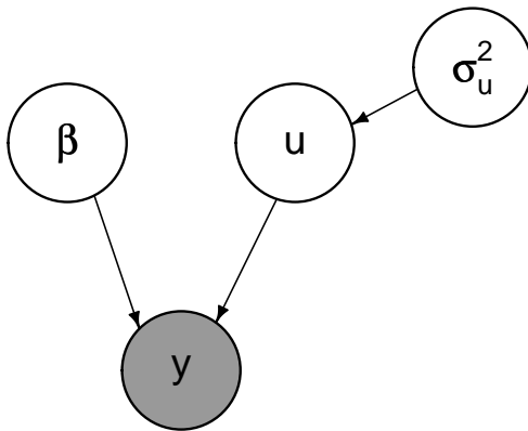
Figure 1: Directed acyclic graph representation of model (4). The shaded node corresponds to the observed data.
