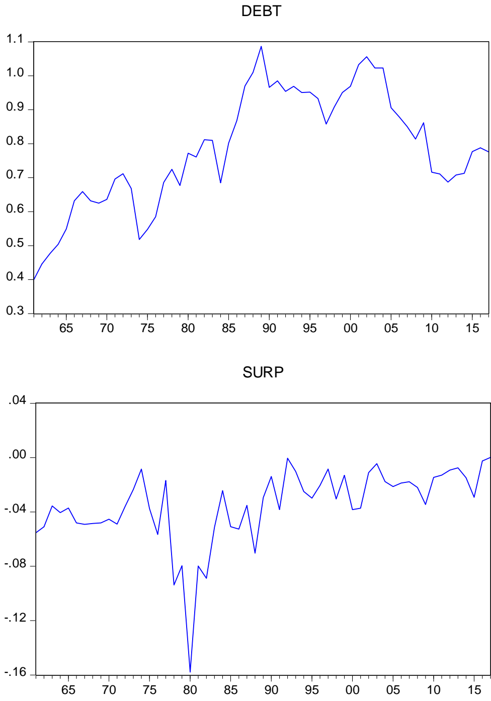
Figure 1. Debt-GDP ratio (DEBT) and Primary Surplus-GDP ratio (SURP) (1961-2017)
