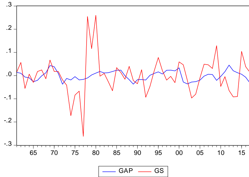
Figure 2. HP filtered output gap (GAP) and cyclical real public spending (GS) (1961–2017)
